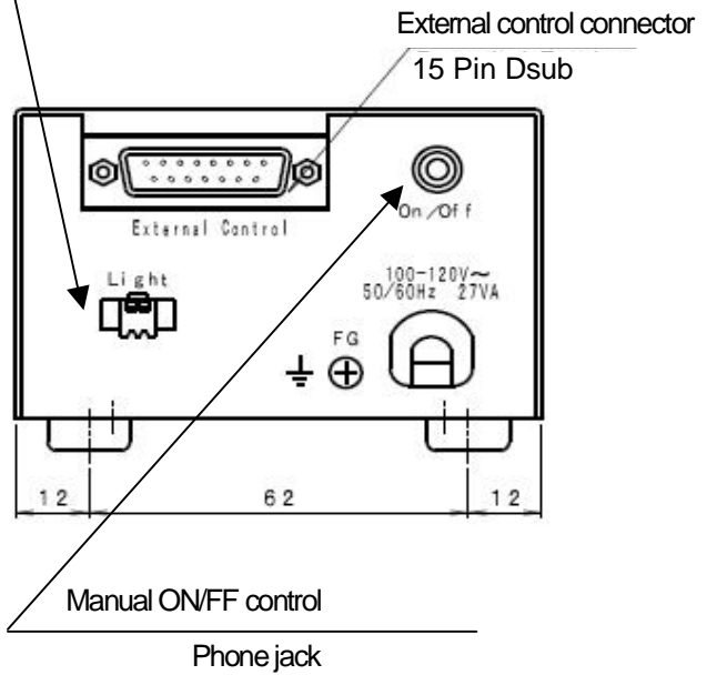
Output Connectors
